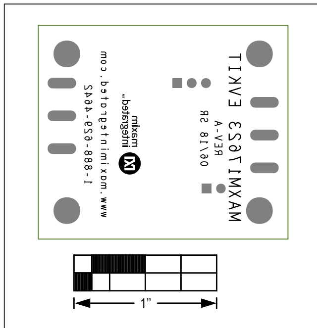
MAXM17623 EV Kit PCB Layout—Silk Bottom
