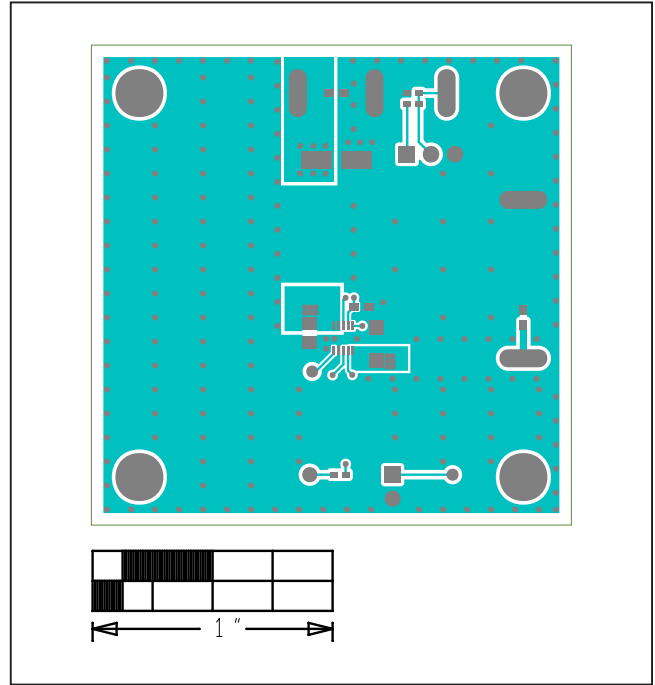
MAXM15464 EV Kit PCB Layout—Top Layer
