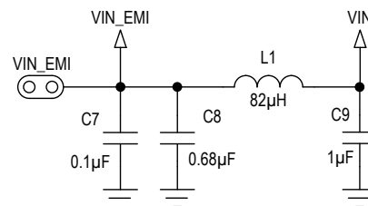
Figure 1. EMI Filter Components
