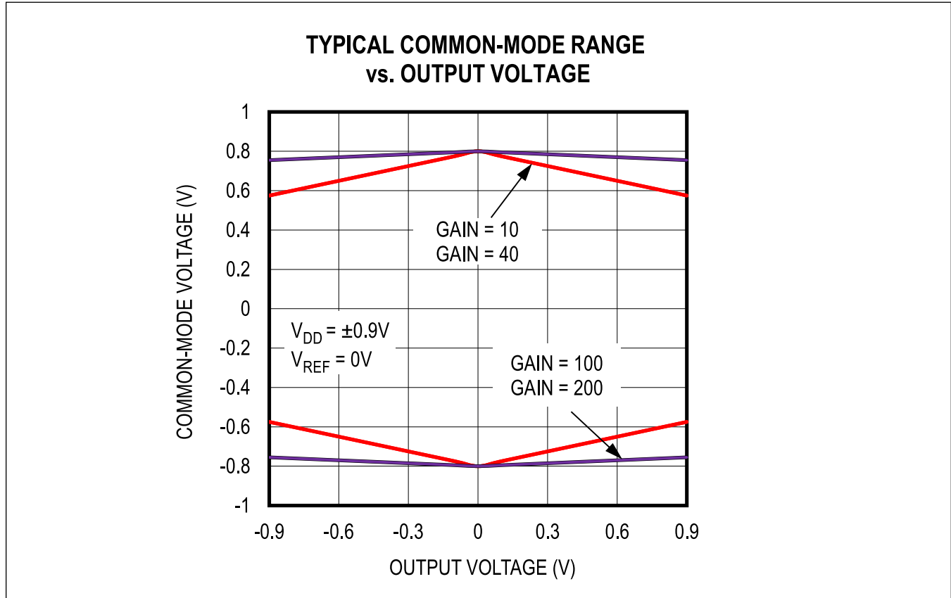
Figure 2. Common-Mode Input Range over Output Swing
