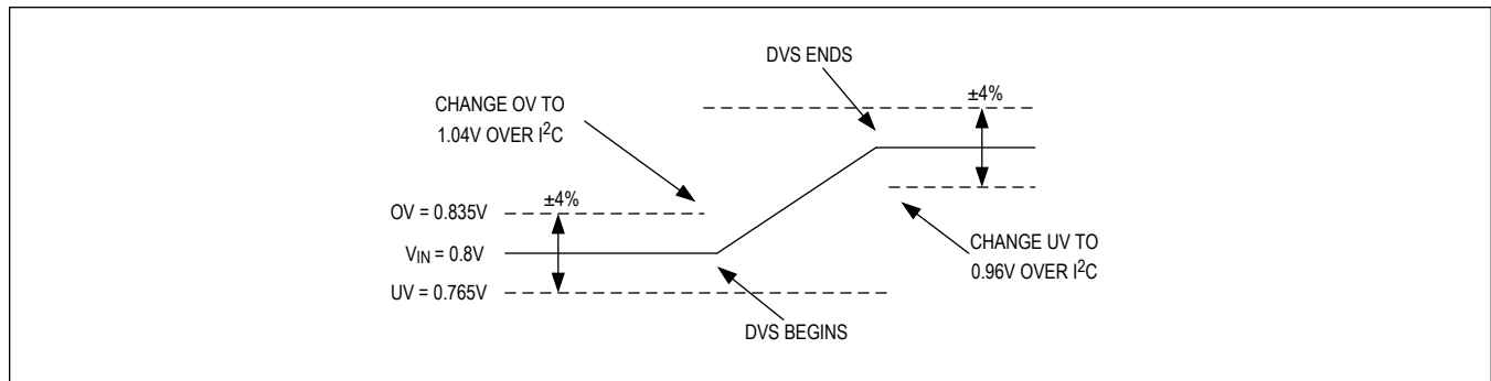
Figure 5. I 2 C DVS Timing Example (Low-to-High Transition)
