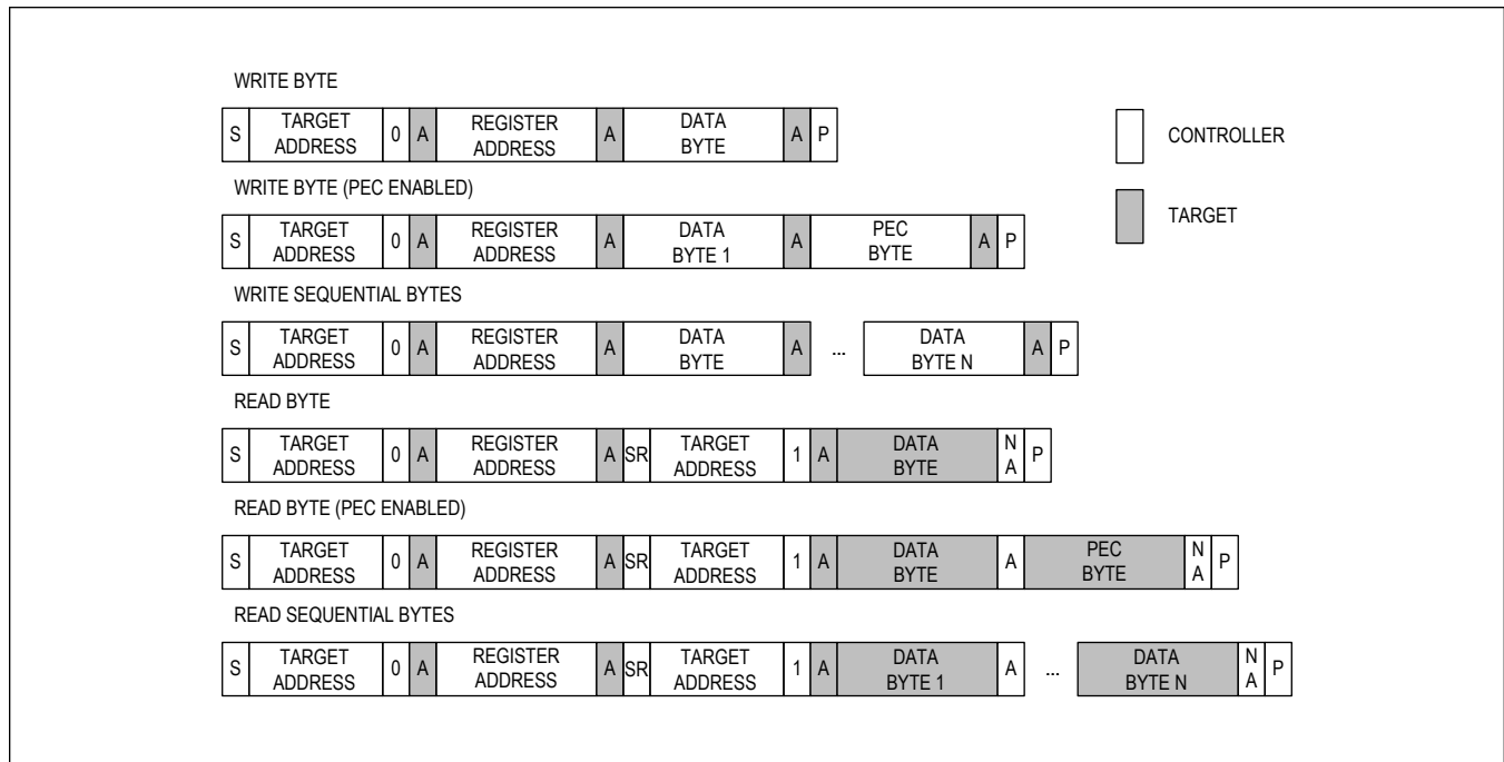
Figure 4. Data Format of I 2 C Interface
