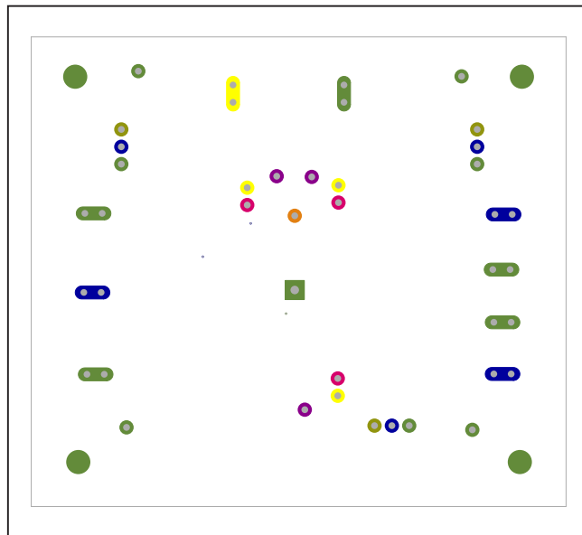
MAX20029B EV Kit Component Placement Guide—Bottom Assembly
