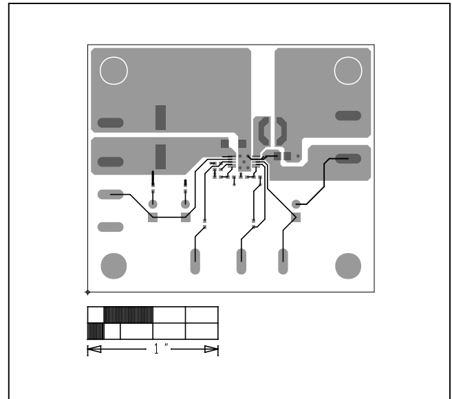
Figure 2. MAX17550 5V EV Kit (μMAX) PCB Layout—Component Side
