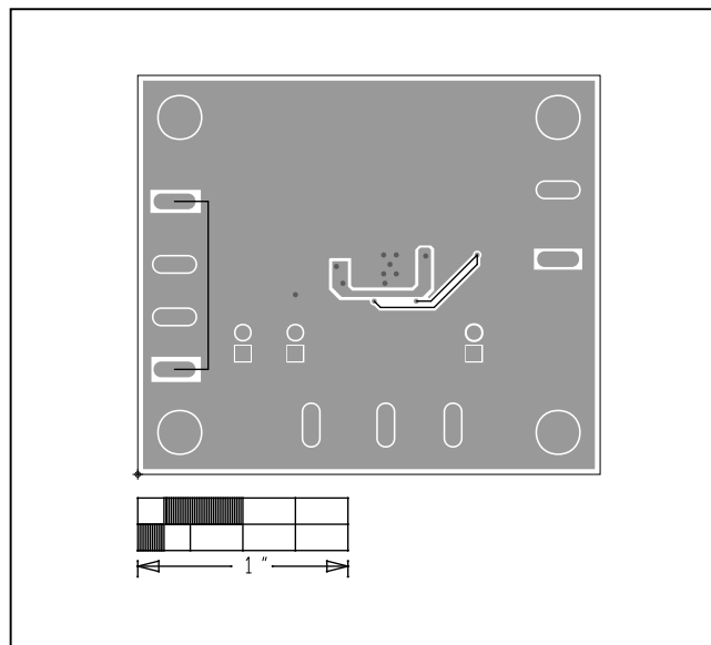
Figure 3. MAX17550 5V EV Kit (μMAX) PCB Layout—Solder Side
