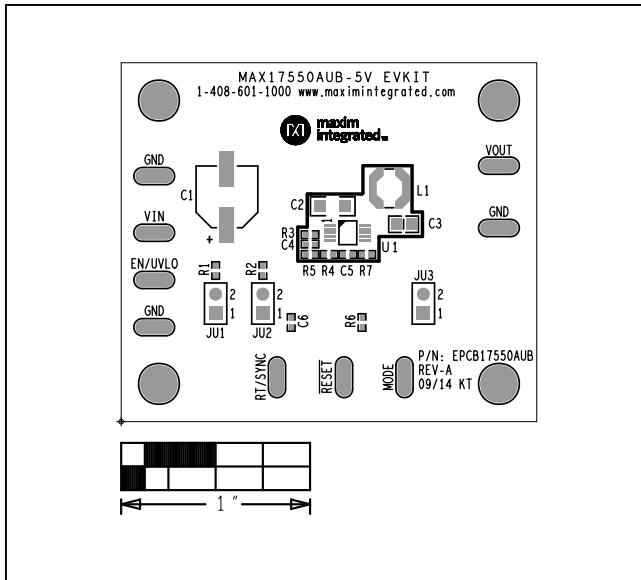
Figure 1. MAX17550 5V EV Kit (μMAX) Component Placement Guide—Component Side
