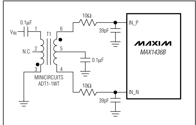
Figure 10. Transformer-Coupled Input Drive
